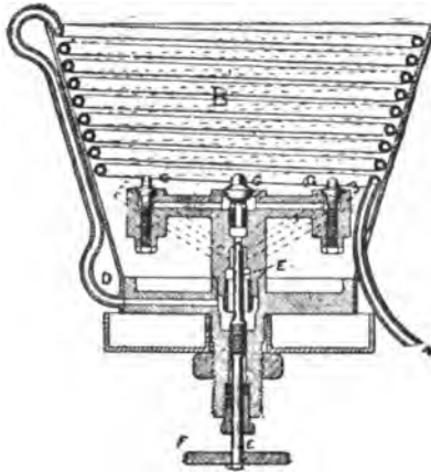
FIG. 203.—The Longuemare Kerosene Vapor Burner. A is the oil feed pipe; B , the vaporizing coil; D , the tube leading to the burner tips; E , the control valve; F , the hand-wheel for regulating the control valve; G, G, G , the burner tips and glands.
